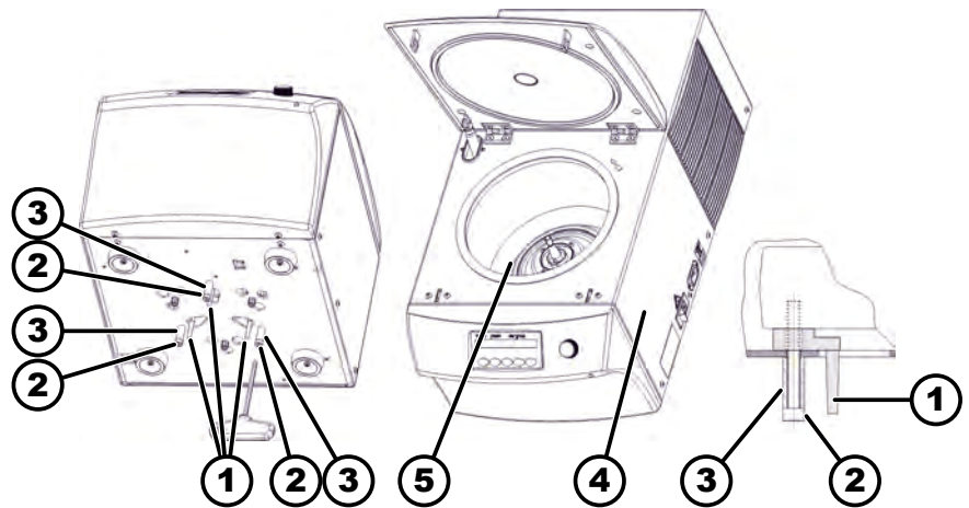
Fig. 14: Transport lock
