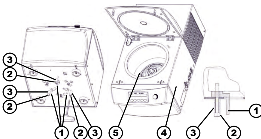
Fig. 13: Transport lock
