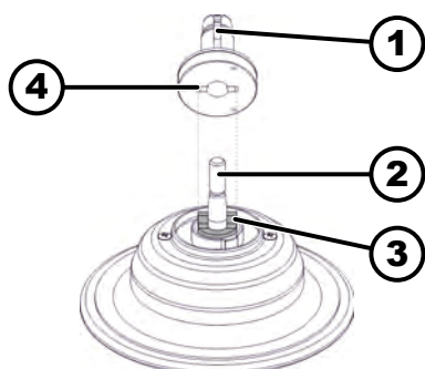
Fig. 17: Hub installation and removal
