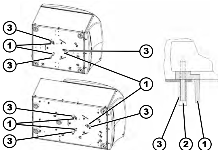
Fig. 14: Transport lock
