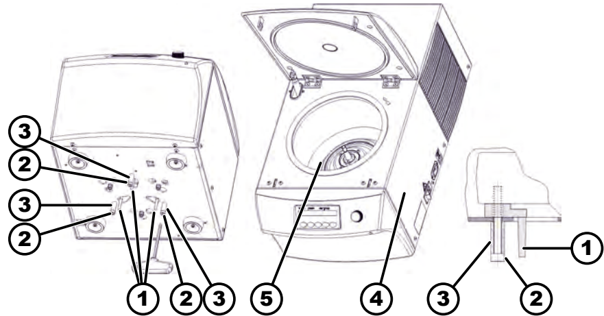
Fig. 14: Transport lock
