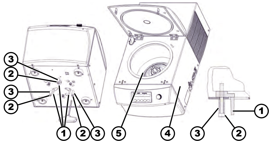
Fig. 13: Transport lock
